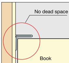
Installation SPF-20
